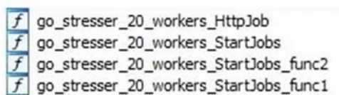
Figure 23: DDOSIA reference
